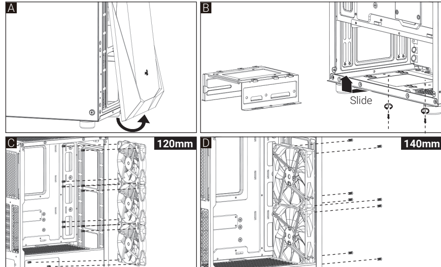
(6a) Install Front Fans
