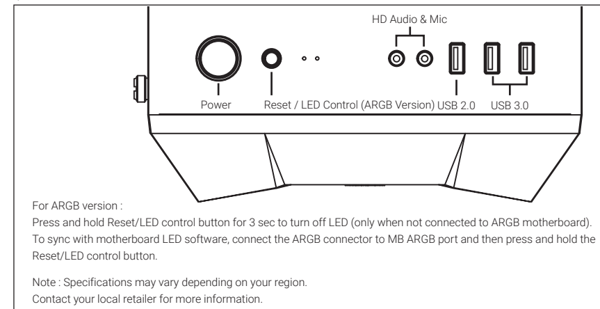
I/O Panel
